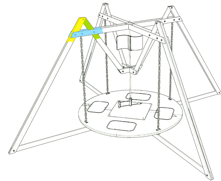
TOP "M" JOINT
